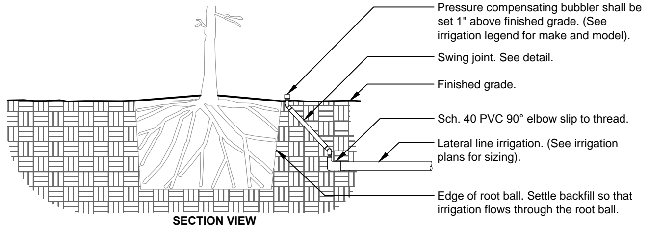
SECTION VIEW
